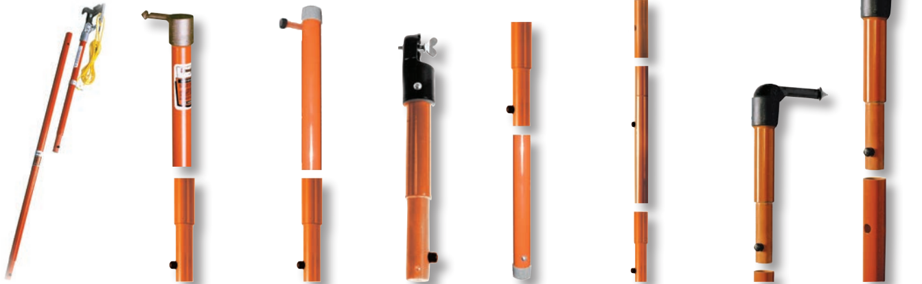
Tree Trimmer Standard Switch Head Disconnect Non-Metallic Disconnect Plastic Universal Base Cap Extension Sections (Both Sizes: 4', 6', 8' and 10' lengths, with female fitting at top and male fitting at bottom) Standard Disconnect Standard Universal
