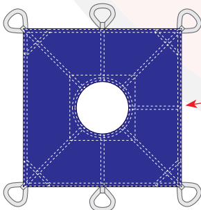
Overlapping Slit with Hook-Loop Fastener & Quick Release Buckles
