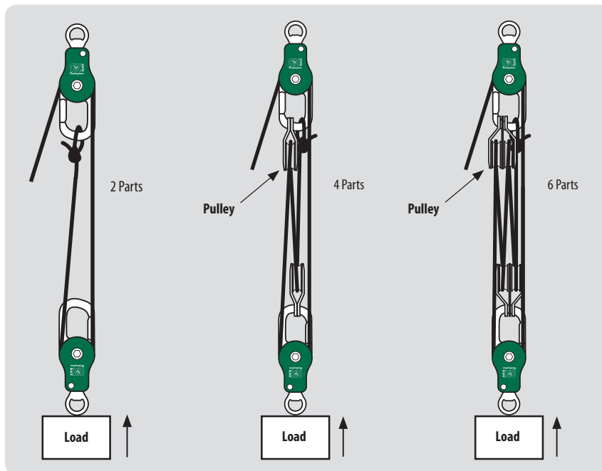
Figure 4: Raising Load
