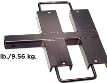
1,000 lb. rating Hitch-Receiver Mount P/N 9700-40980 T3080999 as furnished
