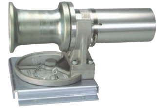
PSC3081563 Hitch Mount Bracket P/N 9700-40980 T3080999 with Swivel Base P/N 9701-23853 (T3081506)
