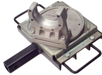
PSC3081563 Hitch Mount Bracket P/N 9700-40980 T3080999 with Swivel Base P/N 9701-23853 (T3081506)
